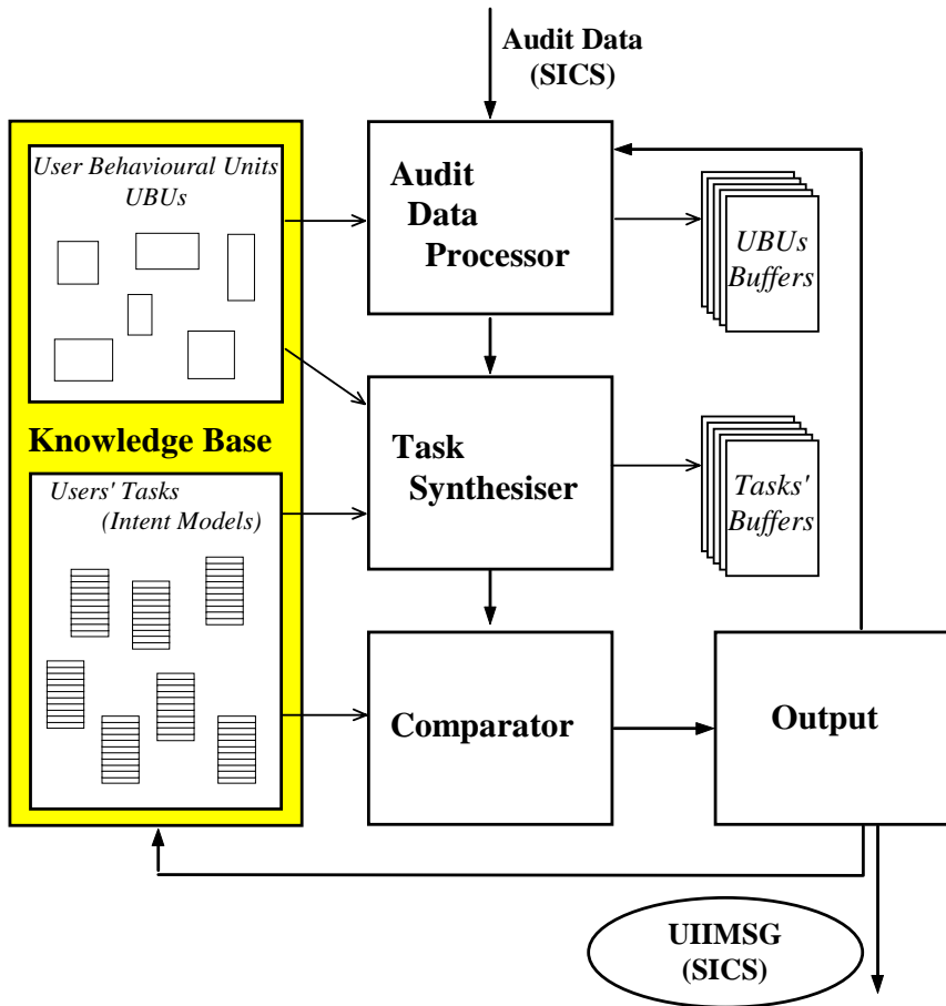
Figure 2. Architecture of the UII module
